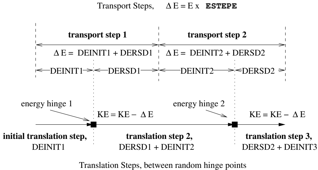
Figure 2.13: Translation steps and transport steps for energy loss hinges. The top half of the figure illustrates the step size (in terms of energy loss) for consecutive conventional Monte Carlo transport steps, with the energy loss set at a constant fraction of the current kinetic energy ( E times ESTEPE , for example). The lower schematic shows how these steps are broken into a series of translation steps between randomly determined hinge distances. Transport through the translation steps is mono-energetic, with full energy loss being applied at the hinge points. Note that the second translation step, for which the electron kinetic energy is constant, actually involves moving the electron through pieces of 2 different transport steps. Multiple scattering could interrupt this energy step translation at any point or at several points, but does not impact the energy transport mechanics.
