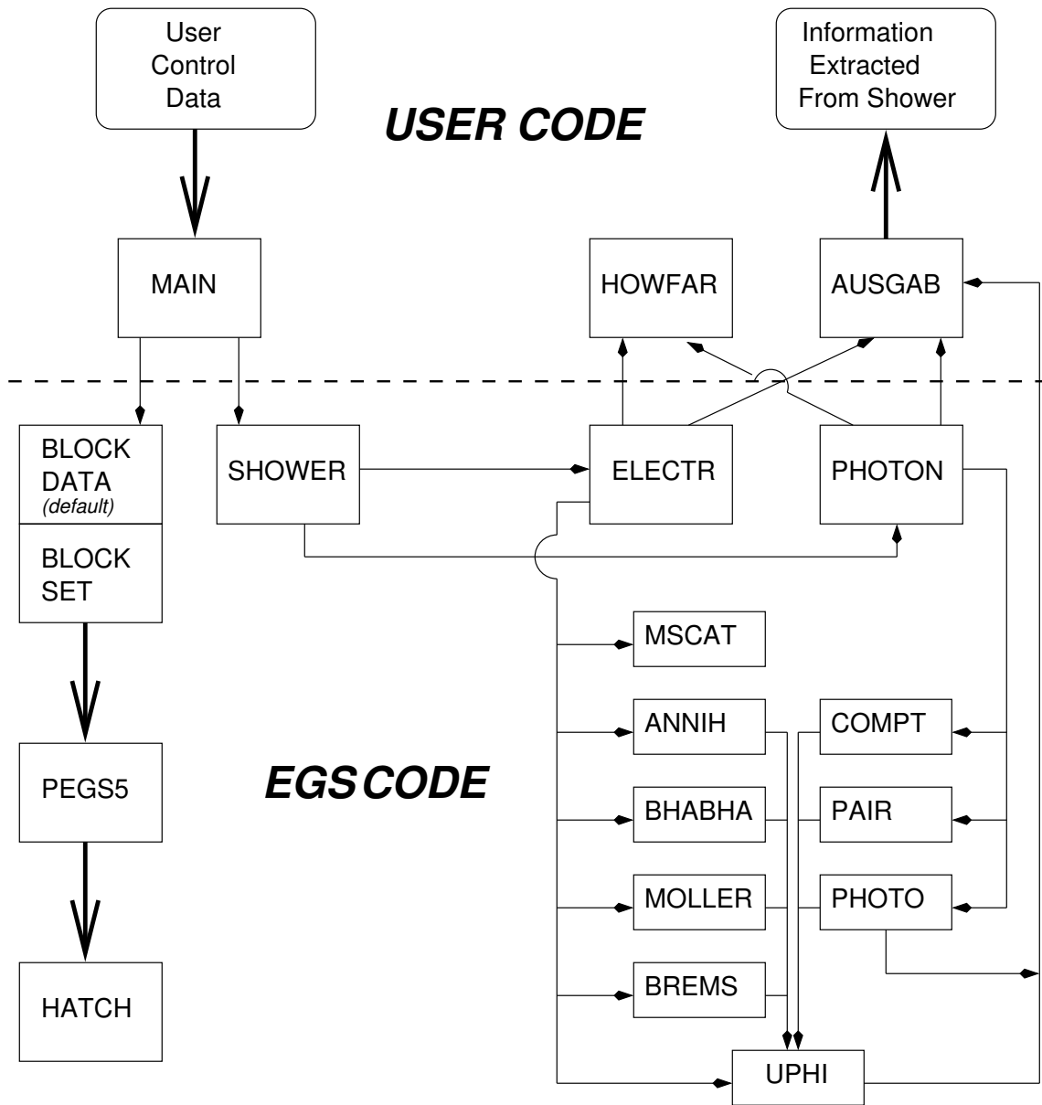
Figure 2.1: Program flow and data control in EGS5.
