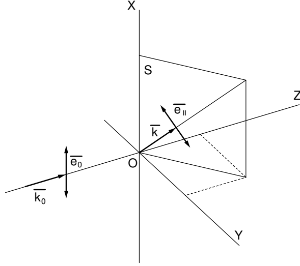
Figure 2.22: Direction of the polarization vector of the scattered photon. Plane S contains \vec{e} and \vec{k} . \vec{e}_{\parallel} is in plane S, and is perpendicular to \vec{k} . \vec{e}_{\perp} is perpendicular to plane S.
