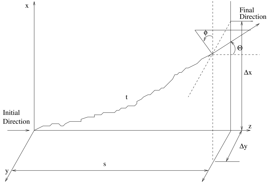
Figure 2.8: Schematic of electron transport mechanics model.
